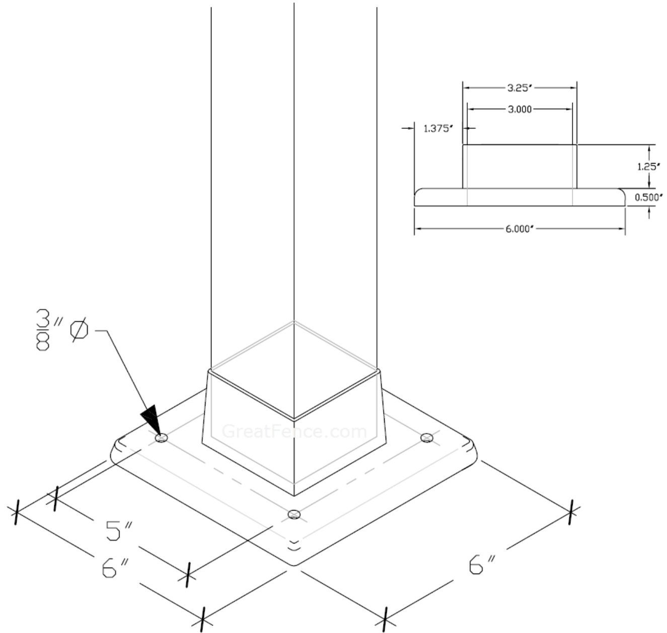
External Deck Mount
